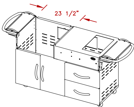
3 BURNER GRILL
