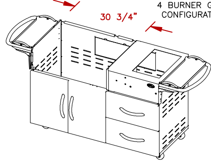
4 BURNER GRILL
