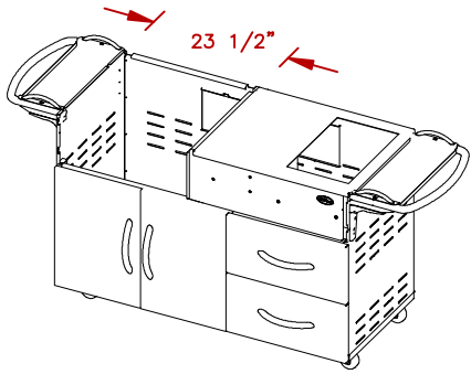
3 BURNER GRILL
