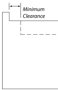
Side view of enclosure with back splash
